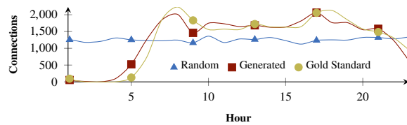
Figure 10. Connections per hour for the Belgian railway case.
