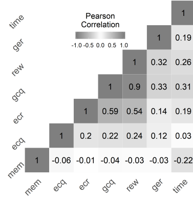
Fig. 9. Correlation matrix with different performance parameters for the TRAVEL ontology.
