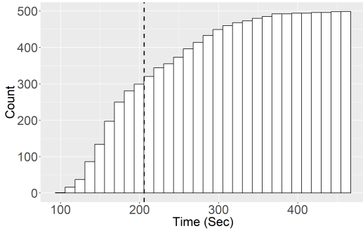
Fig. 7. Cumulative distribution of the time that takes the computation of the rewritings for the TRAVEL ontology.
