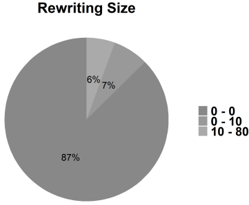
Fig. 5. Size of the rewritings for the TRAVEL ontology.
