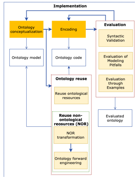
Fig. 4. Public Bus Transport Ontology. Adaptation of LOT Implementation Stage. The "Ontology reuse" activity is expanded and the "Evaluation through Examples" has been added to the Evaluation activity.
