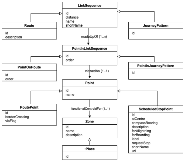
Fig. 8. NOR Transformation of Transmodel UML Network building blocks: points, points in link sequences and link sequences.
