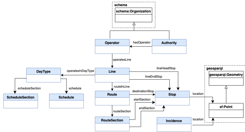
Fig. 6. Public Bus Transport Ontology. Initial Conceptual Model.
